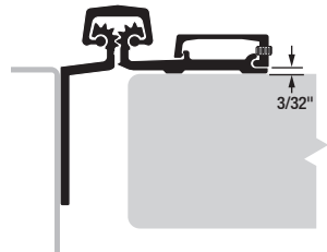
SAFETY HINGE APPLICATION
